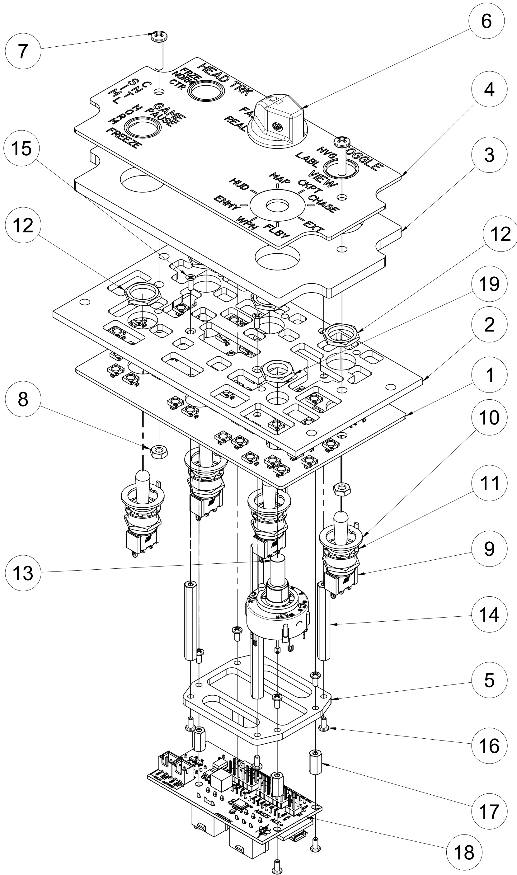
-1 ASSY
